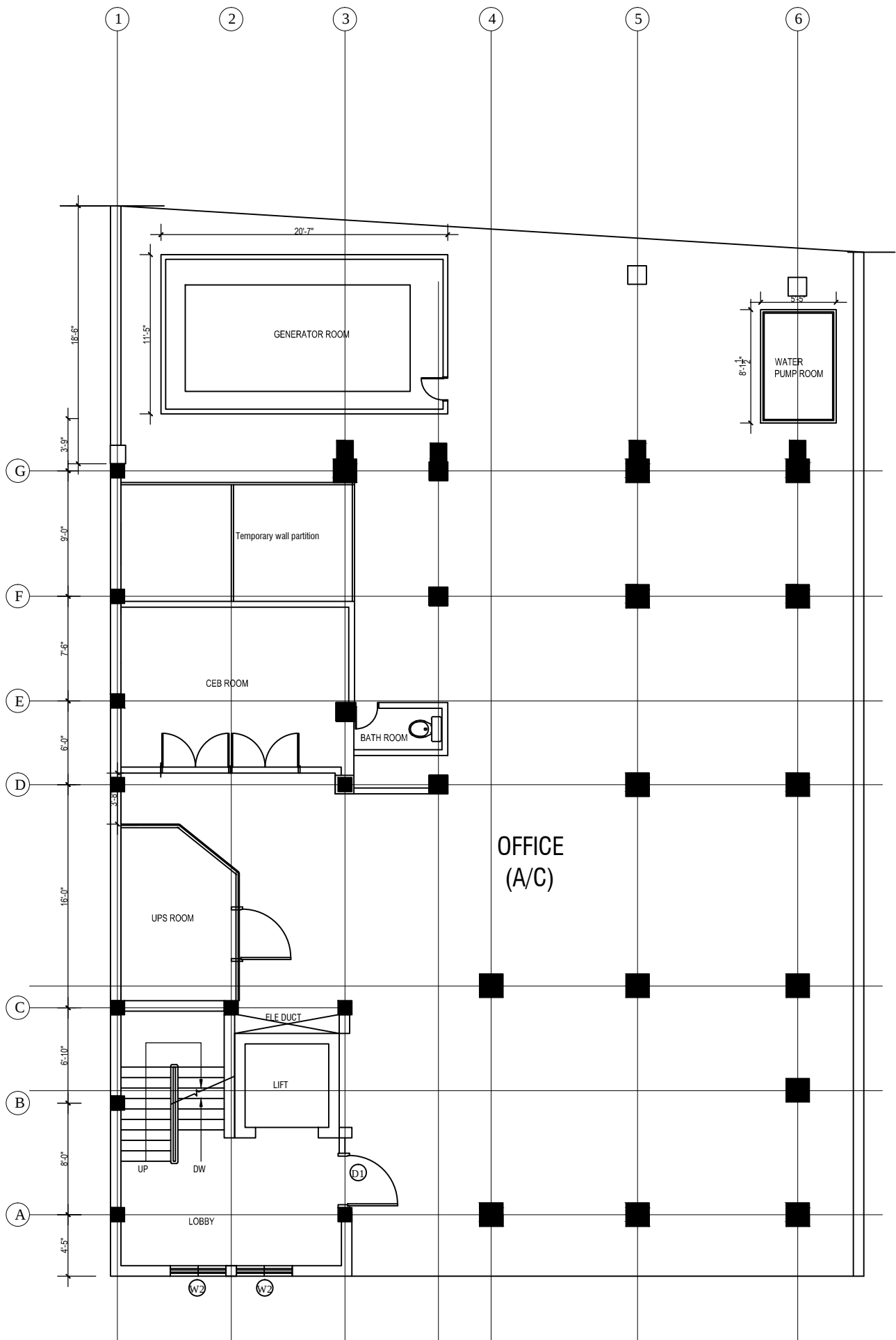
Ground FLOOR
