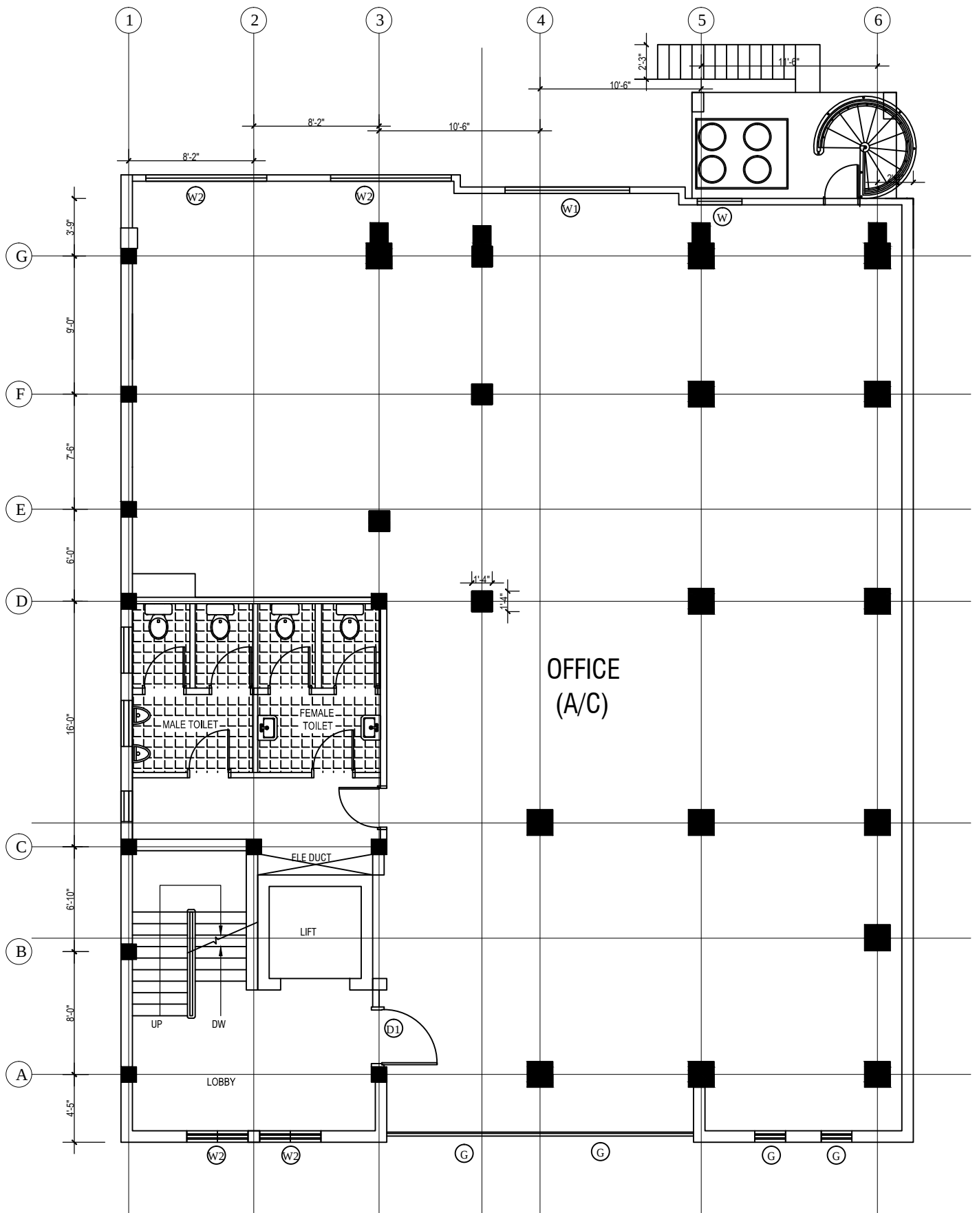
1st FLOOR
